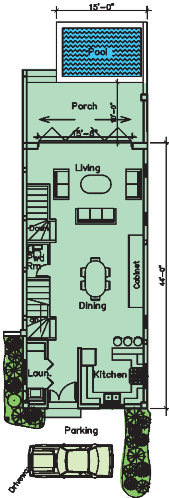
GROUND FLOOR LAYOUT
